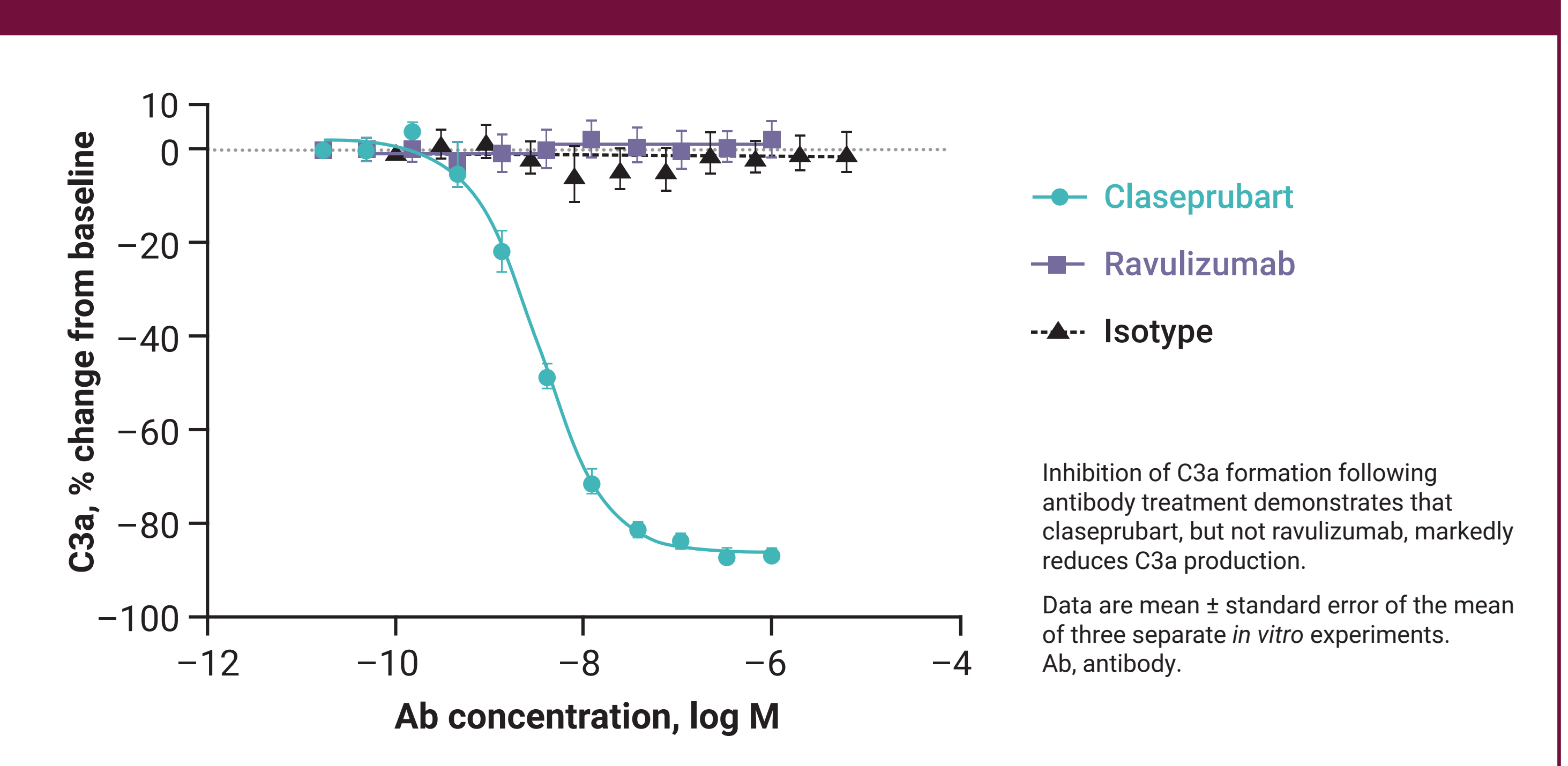
Figure 3. C3a Formation.
