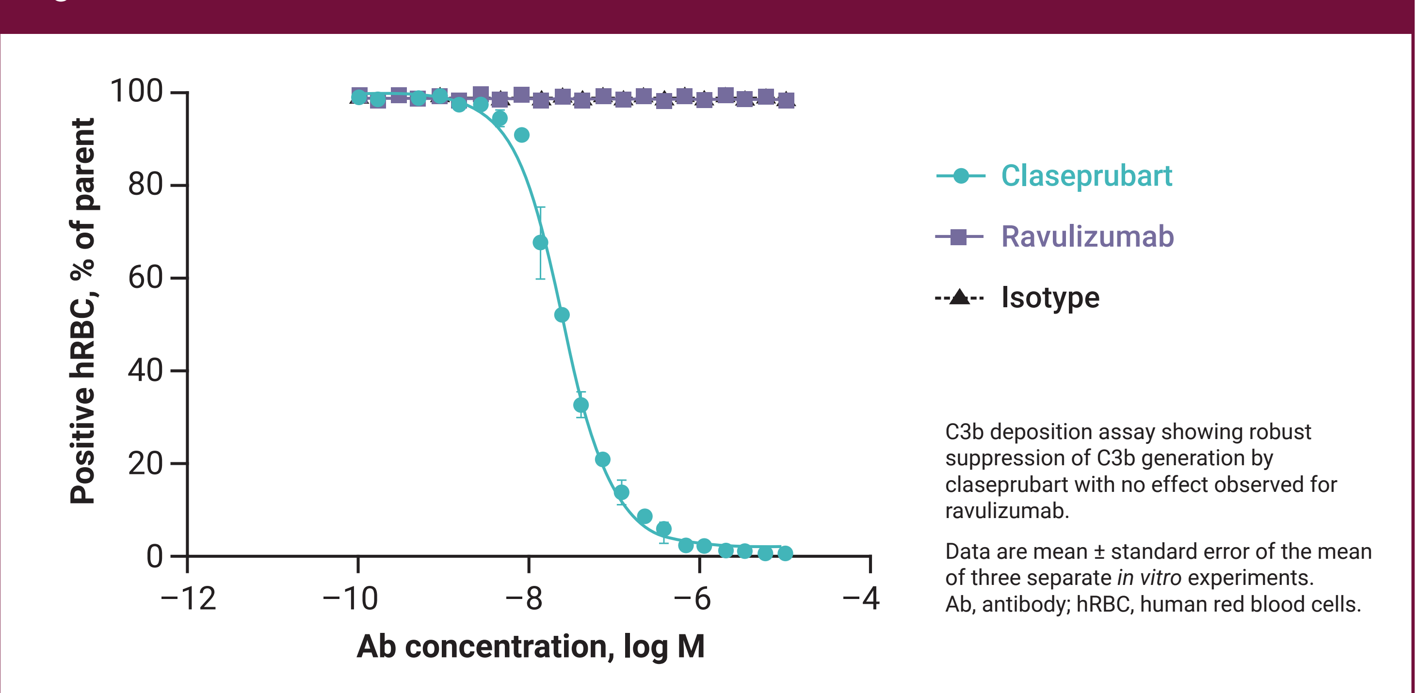
Figure 4. C3b Formation.
