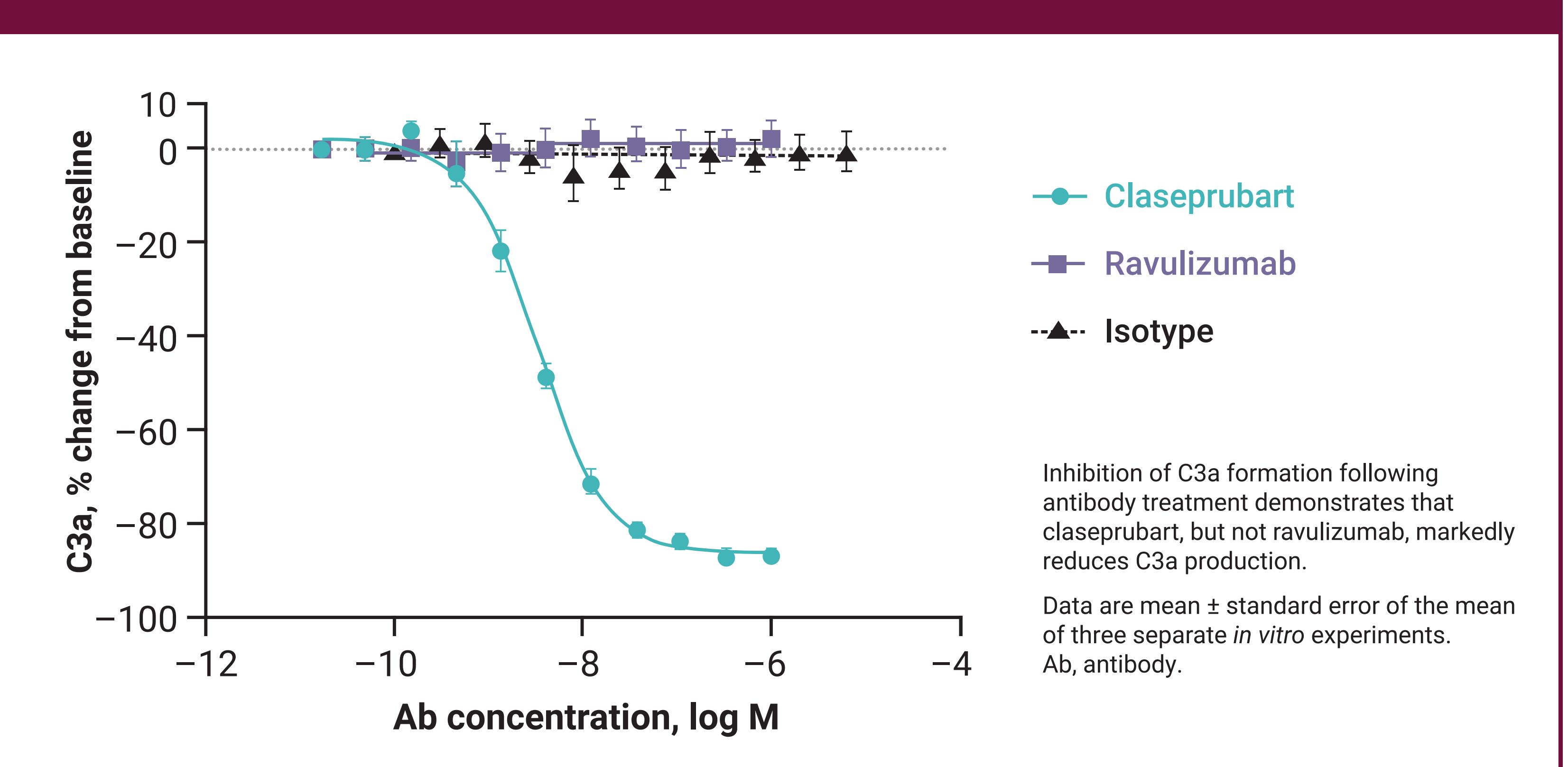
Figure 3. C3a Formation.
