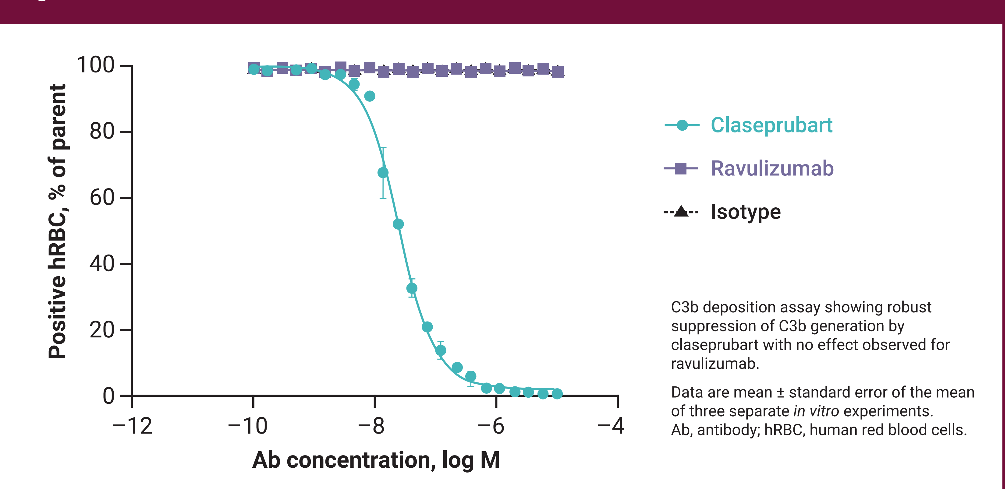
Figure 4. C3b Formation.
